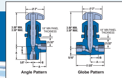
Needle Valves
