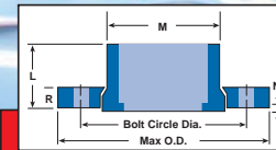
Van Stone-Style Flange (Soc - Two Piece)
